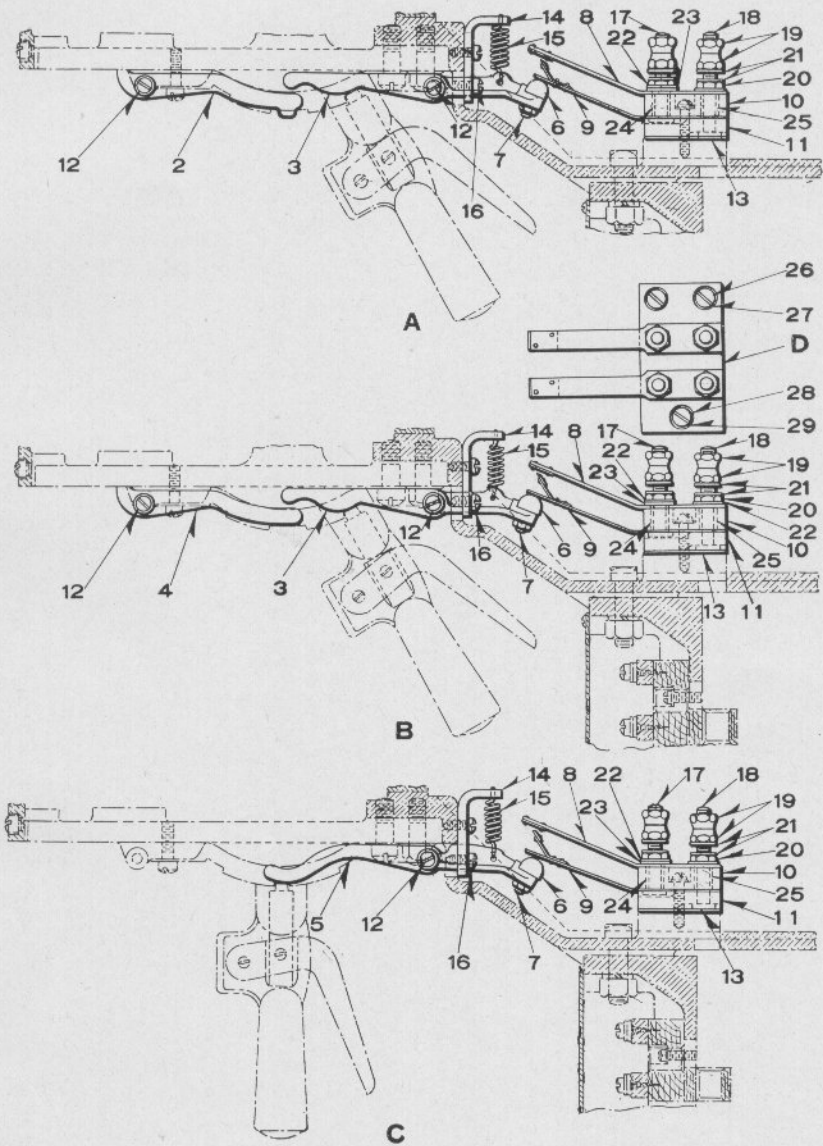
LATCH CIRCUIT CONTROLLERS WITH TWO CONTACTS
